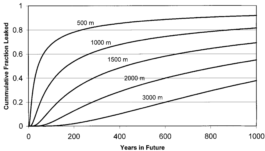
Figure 1. Leakage over time as a function of injection depth.
