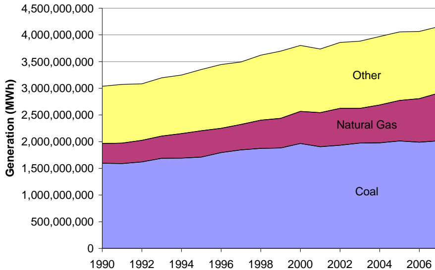
Figure 2-2. Electricity Generation by Source 1990-2007 2
