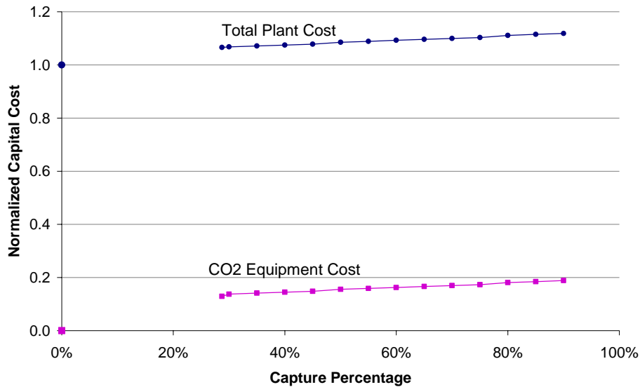
Figure 9-3. Capital Cost Dependency on Capture Percentage for IGCC Model
