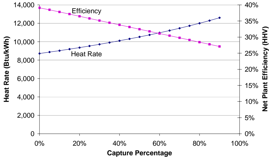
Figure 8-2. Plant Performance Dependency on Capture Percentage for SC PC Model
