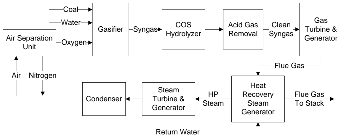
Figure 5-4. Simplified Process Flow Diagram of an IGCC Power Plant 189
