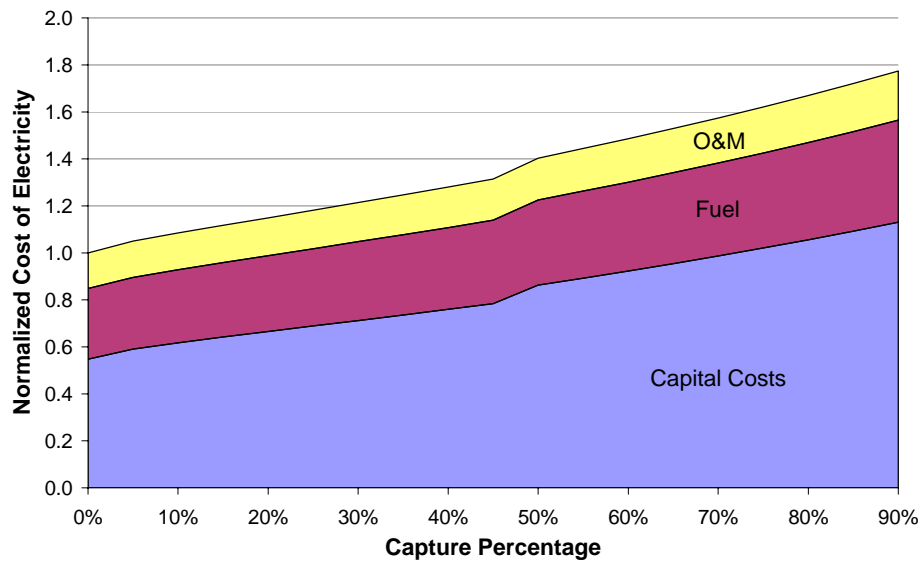
Figure 8-5. Cost of Electricity Dependency on Capture Percentage for SC PC Model
