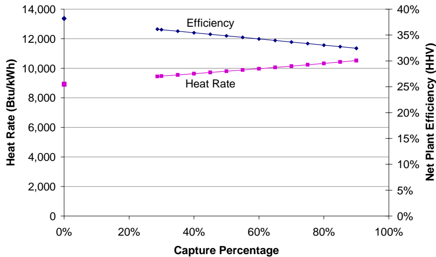
Figure 9-2. Plant Performance Dependency on Capture Percentage for IGCC Model
