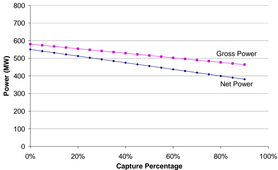
Figure 8-1. Plant Output Dependency on Capture Percentage for SC PC Model
