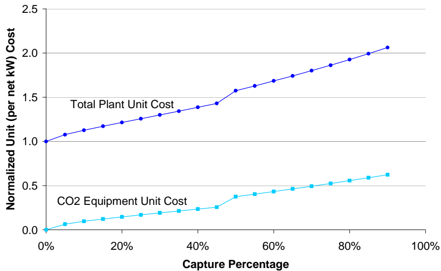
Figure 8-4. Unit Cost Dependency on Capture Percentage for SC PC Model
