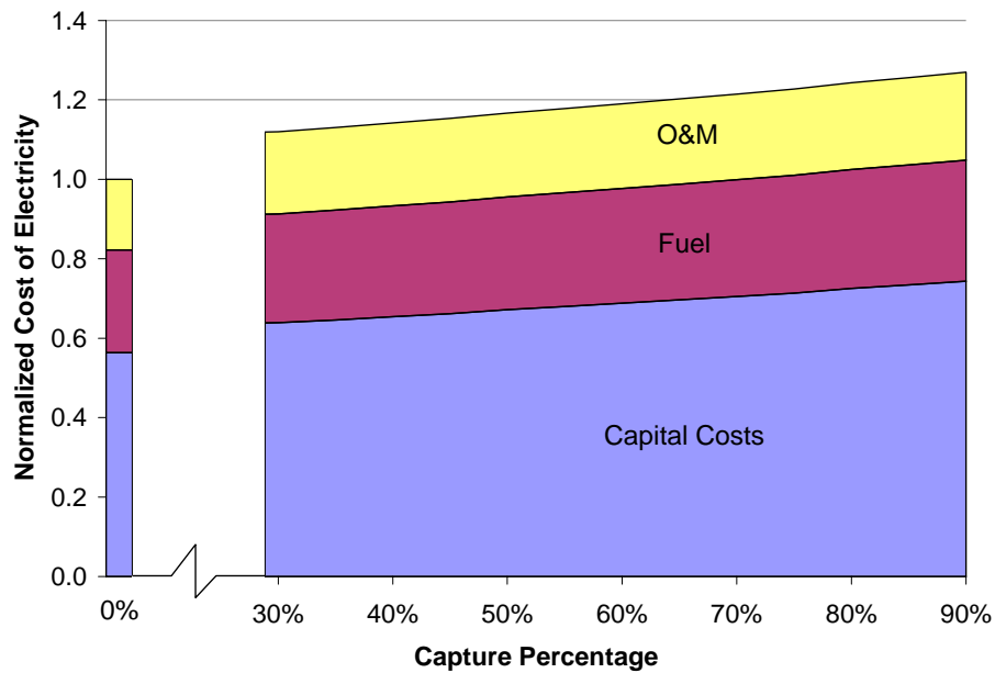
Figure 9-5. Cost of Electricity Dependency on Capture Percentage for IGCC Model
