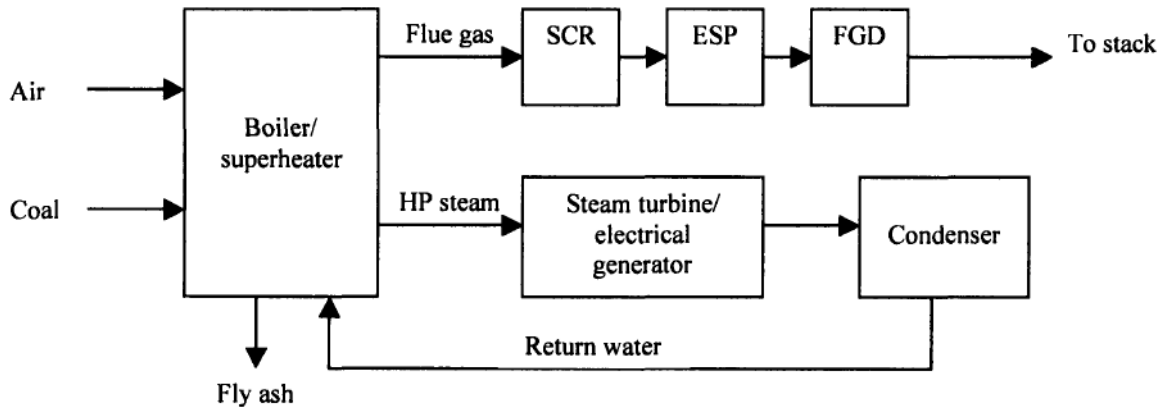
Figure 5-1. Simplified Process Flow Diagram of Pulverized Coal Power Plant 179
