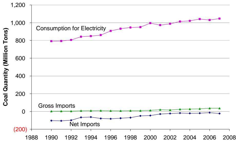
Figure 2-4. Coal: Consumption for Electricity and Imports 5
